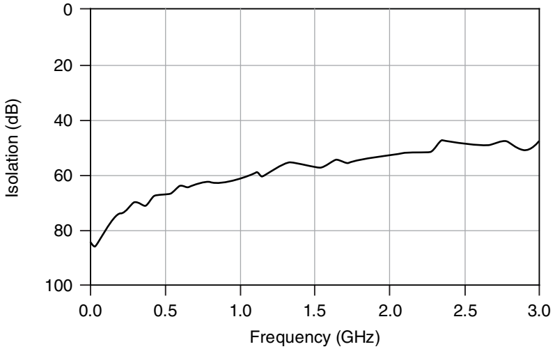
Figure 4. Isolation, Typical
